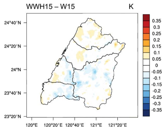
(c) Temperature at 2m
